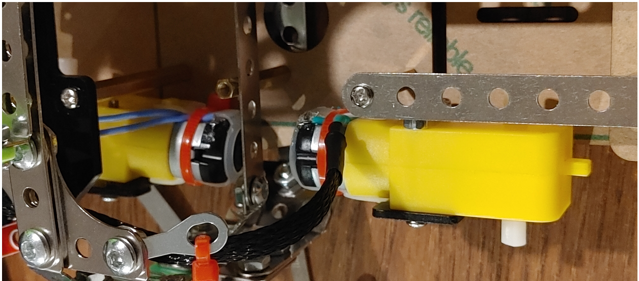
Fig. 3: DC Motors wires secured inside harnes.
