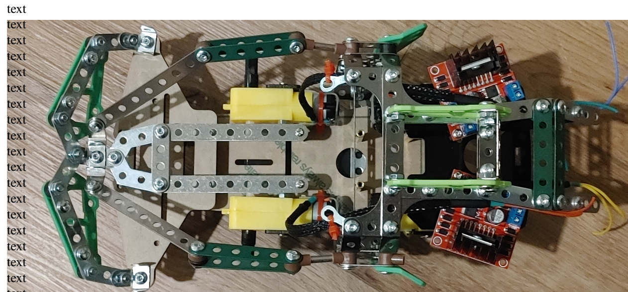
Fig. 1: Completed chassis with only DC motor controllers installed.
